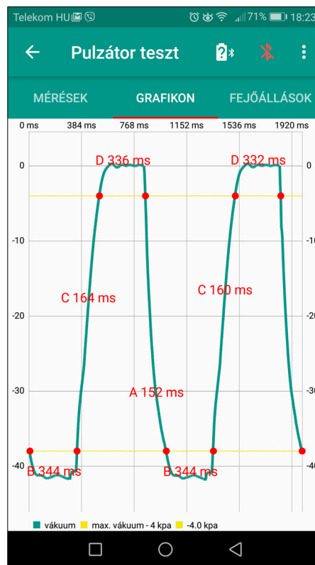
Pulsation curve characterising a dirty pulsator valve
